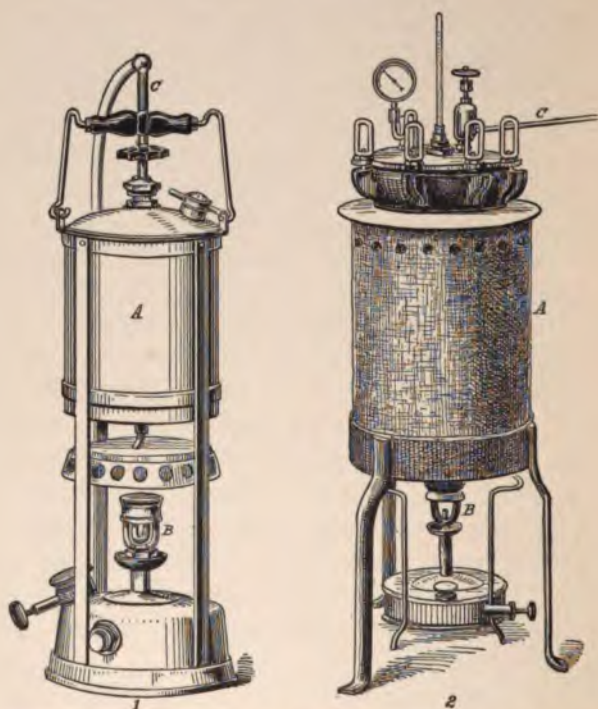
FIG. 5.—Autoclaves for generating formaldehyd (1) from formalin and (2) from formochloral: A , chamber for reception of the fluid; both chambers are hermetically sealed when apparatus is in operation; B , lamp for supplying heat; C , tube for conducting gas from generator into the room to be disinfected (Abbott).
